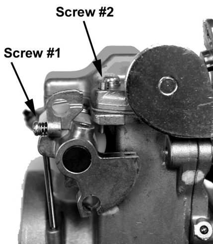
Figure T4 ACCELERATOR PUMP
